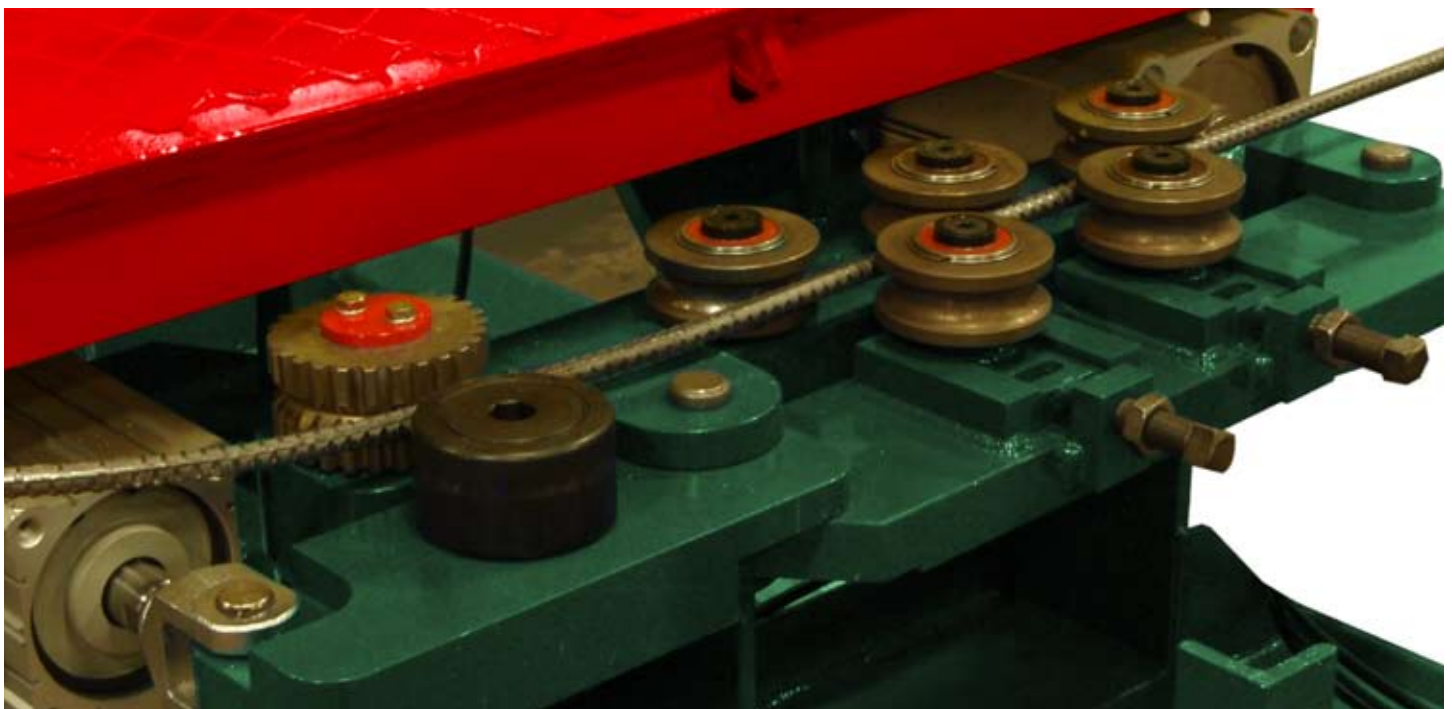
PreStraightener has powered drive to pull bar through straightner and makes loading any automatic easier.
